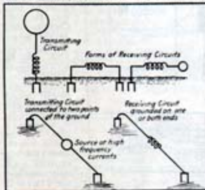
Arrangements of Directive Circuits Described in Tesla's U. S. Patent No. 813,809 of November 8, 1898, on "Method of and Apparatus for Controlling Mechanism of Moving Vessels or Vehicles." Fig. 12.
